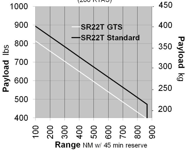
SR22T High Speed Cruise @ 18,000 Ft (200 KTAS)
